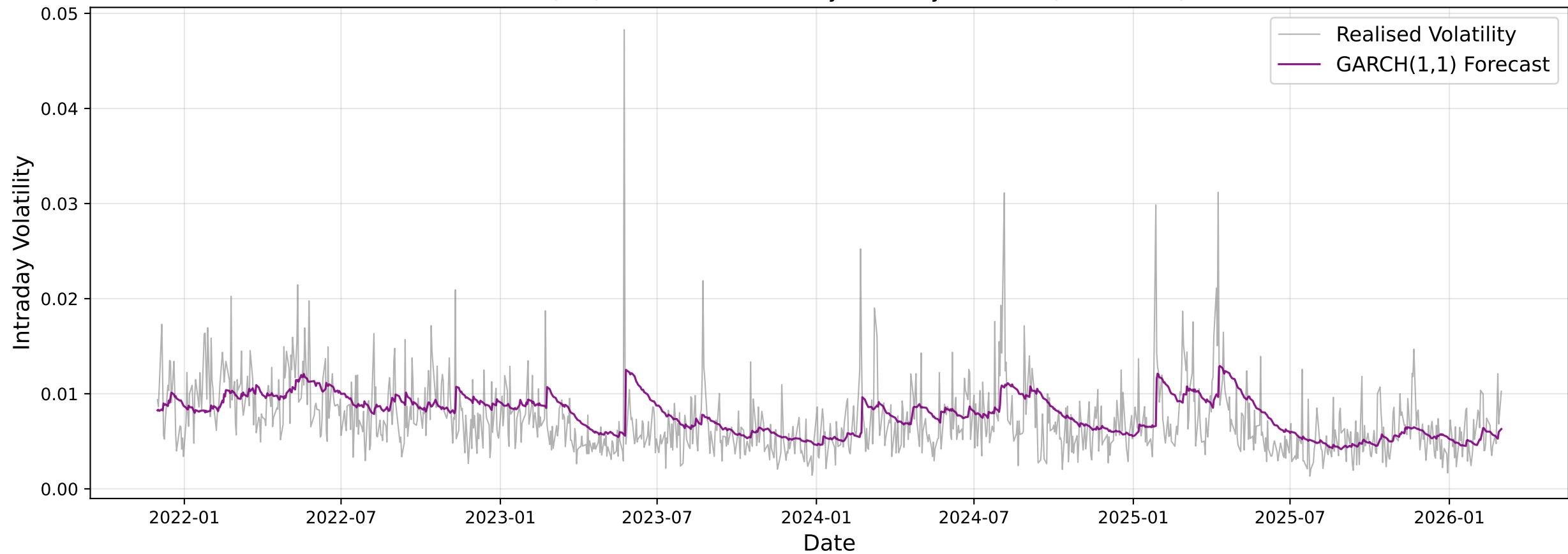
GARCH(1,1) vs. Realised Intraday Volatility — NVDA (Test Period)
